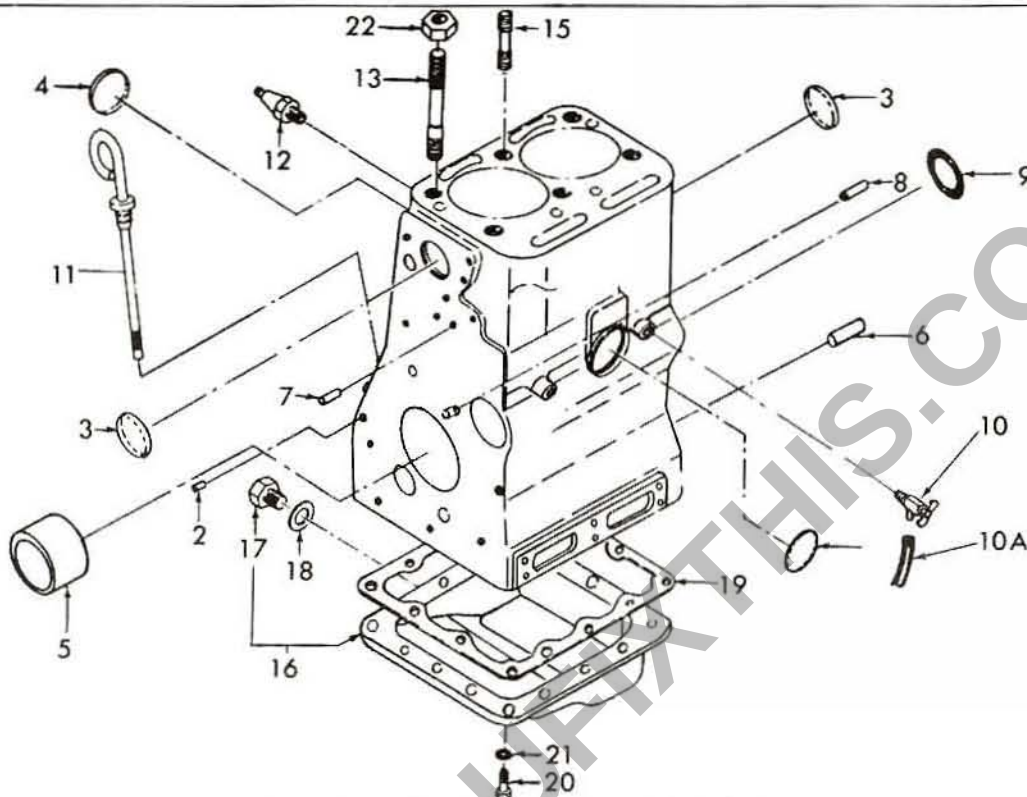
FIG. 6-1 — BLOCK ASSEMBLY, CYLINDER
